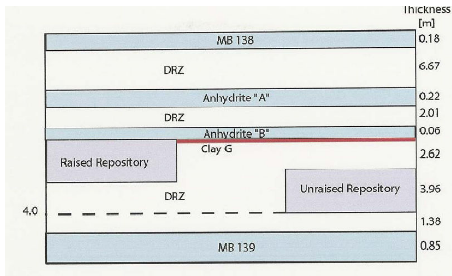
Figure 9-5. Schematic of the Stratigraphy Surrounding the Raised and Unraised Sections of the Repository (Not to scale) (Source: Stein and Zelinski 2003c)
